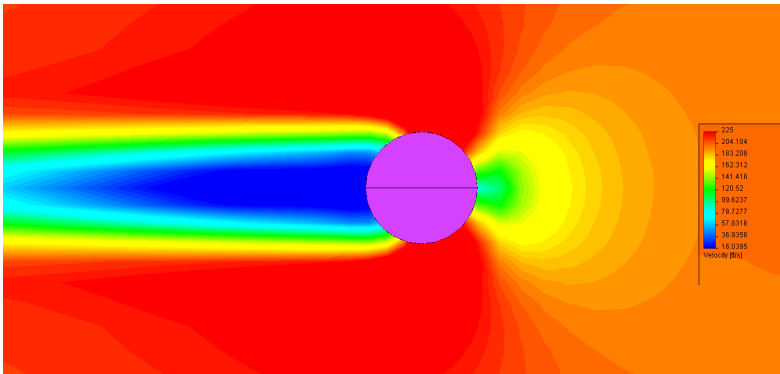
Simulation Design of Flow Around a Sphere
