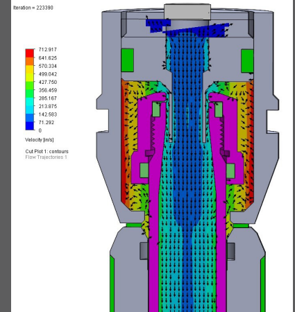
Computational Fluid Analysis of a Centrifuge
